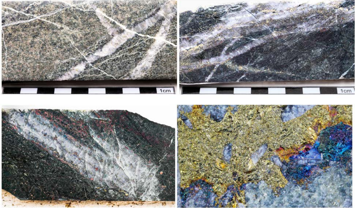
Figure 3: (TOP LEFT) Rock slab PVT0825-001 (184.8m) showing volcanic andesite, strongly kaolinite-chlorite altered and cut by porphyry B-veins with pyrite to chalcopyrite ratio of 5:1 (pyrite shell) - 3-metre sample assayed 0.14% copper and 0.04 g/t gold (0.17% CuEq 1 ). (TOP RIGHT) Rock slab PVT0825-001 (412.0m) showing diorite, strongly magnetite-chlorite altered and cut by cm-scale porphyry B-veins with chalcopyrite to pyrite ratio of 2:1 (chalcopyrite zone) - 3-metre sample assayed 0.89% copper and 0.39 g/t gold (1.17% CuEq 1 ). (BOTTOM LEFT) Rock slab PVT0825-001 showing diorite, strongly biotite altered and cut by cm-scale porphyry B-veins with bornite mineralization (bornite zone) - 2.5m sample assayed 1.14% copper and 1.19 g/t gold (1.98% CuEq 1 ). (BOTTOM RIGHT) Microphotograph showing bornite-chalcopyrite-pyrite mineralization, observed starting at 300m depth.
