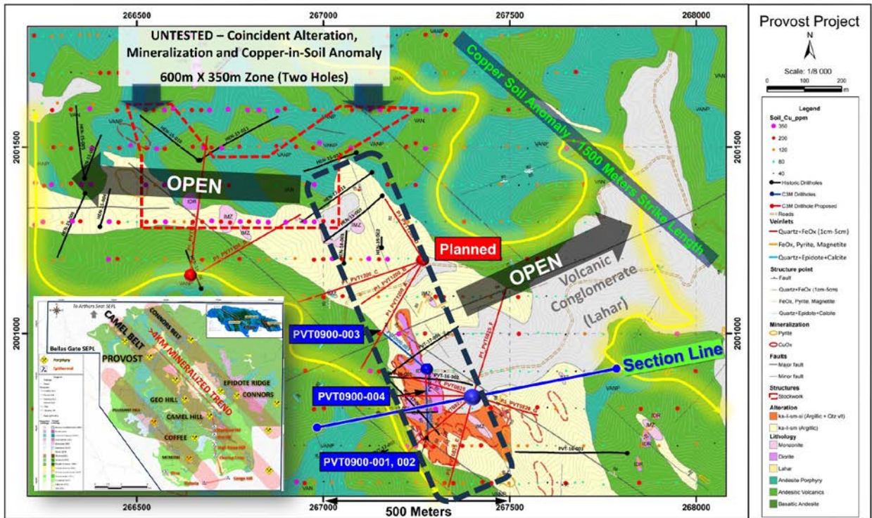
Figure 1: Plan view map of Provost showing historical drill holes in black, recently completed drill holes in blue and planned drill holes in red. Black hash line outlines 900m by 200m initial drill target area. Based on alteration and soil geochemistry, the drill target area remains open in multiple directions and at depth.
