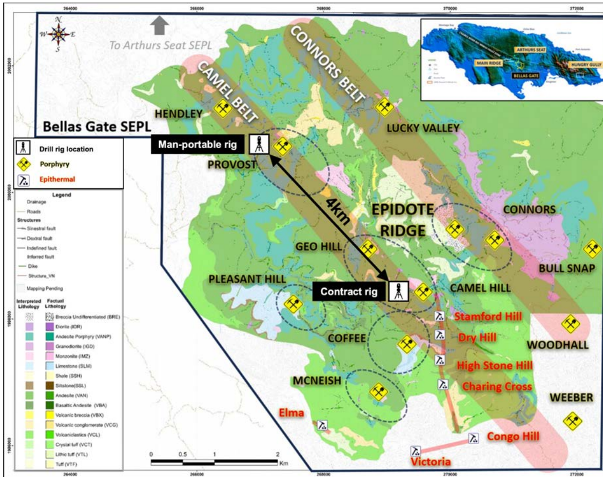
Figure 4: C3 Metals' Bellas Gate project location map showing geology and high priority copper-gold porphyry and epithermal prospects along two porphyry and epithermal copper-gold belts. Note the locations of two drill rigs currently operating.
