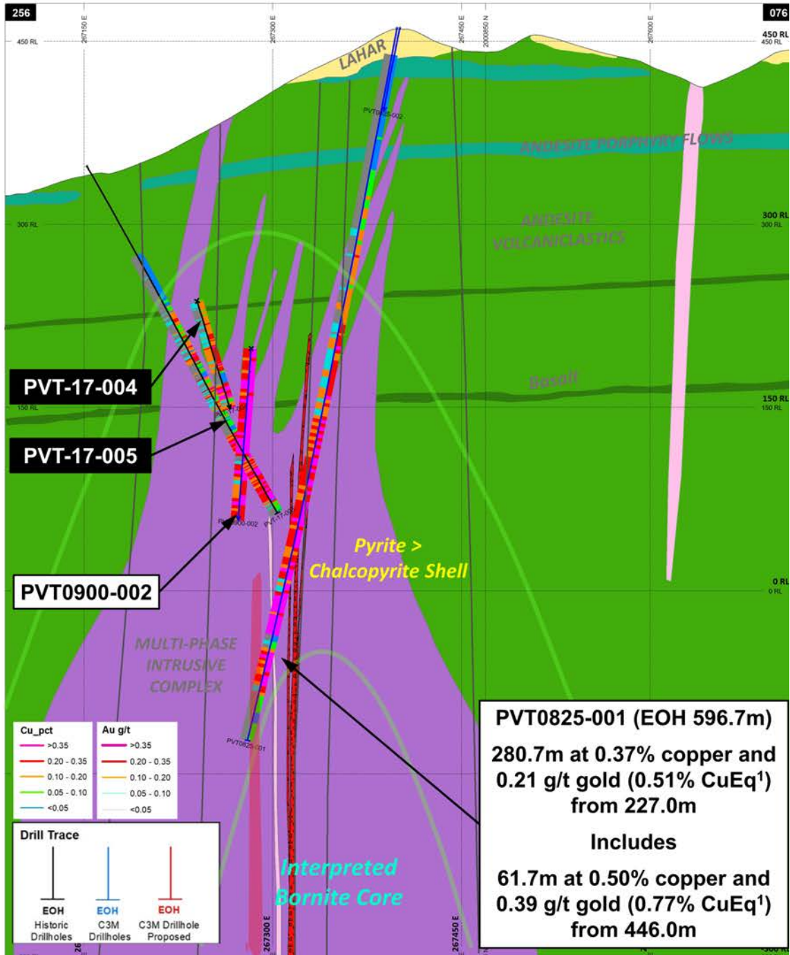
Figure 2: Cross section through PVT0825-001, showing lithology and copper-gold assays.
